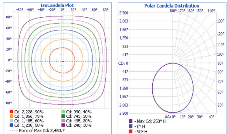
Isocandela Plot
